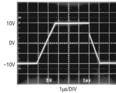
\pm 15V Large-Signal Response
